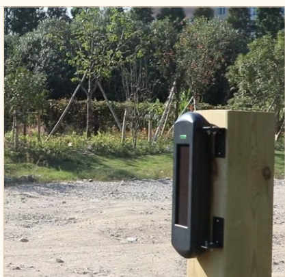
Solar beam sensor on a boundary post, paired unit opposite
